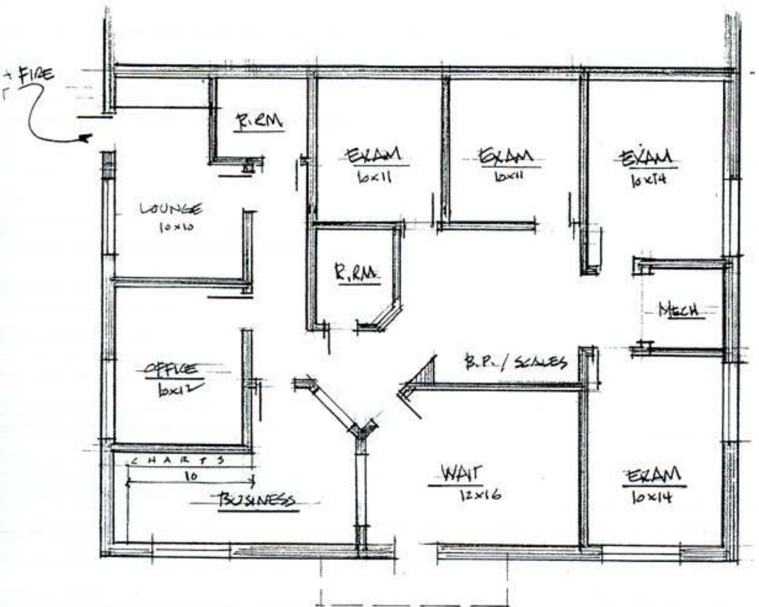
FLOOR PLAN 1/8"=1'-0"
